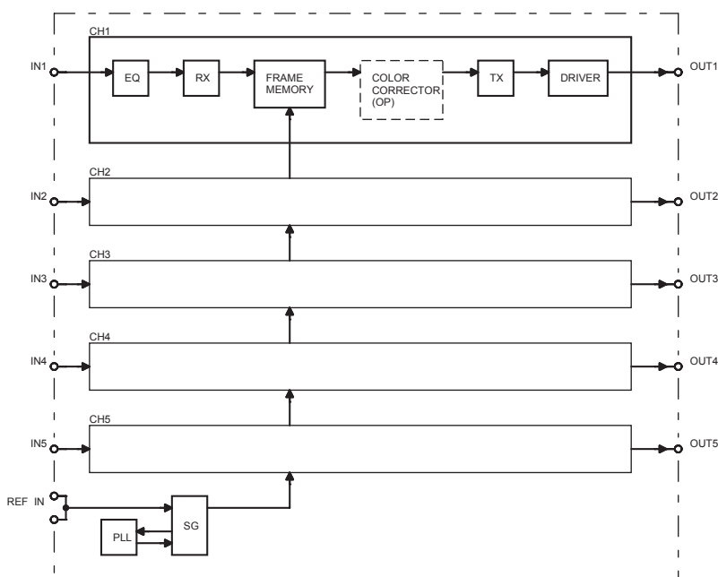
HSI-110F FRAME SYNCHRONIZER BLOCK DIAGRAM
